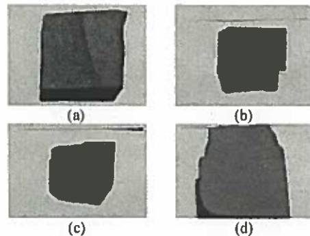
Fig. 6 Red sandstone samples at different cleaning stages: (a) t = 0 s; (b) t = 3 s; (c) t = 6 s and (d) t = 10 s.
