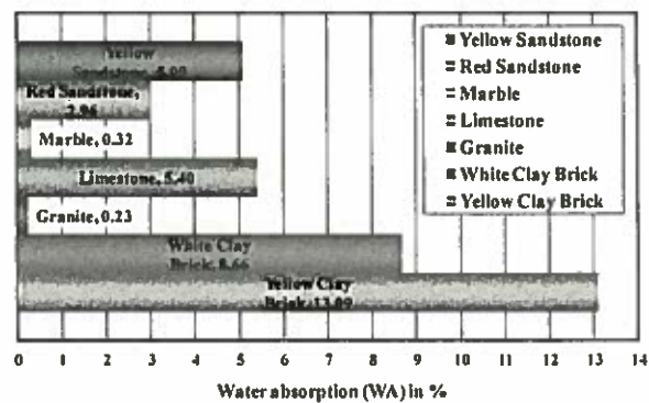
Fig. 29 Water absorption for various types of masonry stones and bricks.
