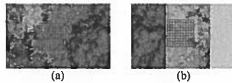
Fig. 18 Grids on the greyscale images of the granite samples: (a) t = 0 s and (b) fresh surface..
