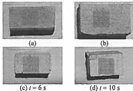
Fig. 16 Grids on the greyscale images of the limestone samples: (a) t = 0 s; (b) t = 3 s; (c) t = 6 s and (d) t = 10 s.
