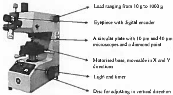
Fig. 23 Vickers hardness instrument.
