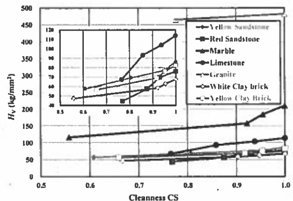
Fig. 27 Vickers hardness number versus cleanness for various masonry stones and bricks.
