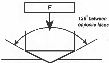
Fig. 24 The pyramid shaped indenter.
