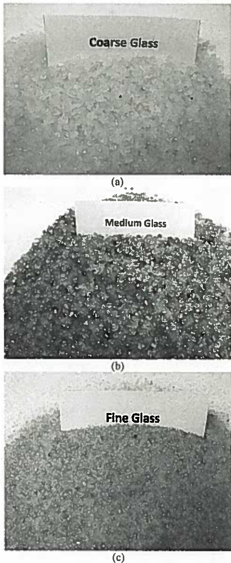
Fig. 3 Recycled glass particles for air abrasive cleaning. (a) coarse glass; (b) medium glass and (c) fine glass.
