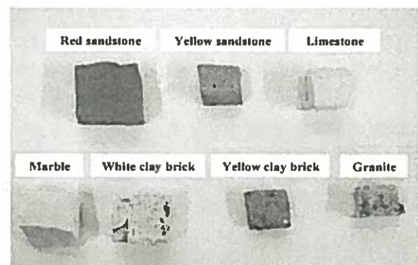
Fig. 28 Masonry stone and brick samples for water absorption tests.
