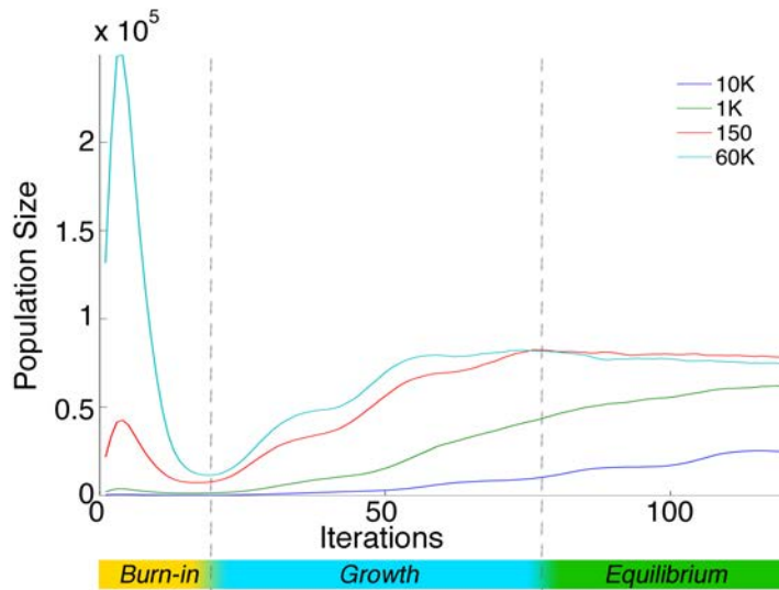
Figure 14. Comparison of the total population size over a 120 year simulation when using different numbers of initial trees (numbers in legend). Different phases of growth are highlighted with a gradient scale (as there is some variation between experiments).
