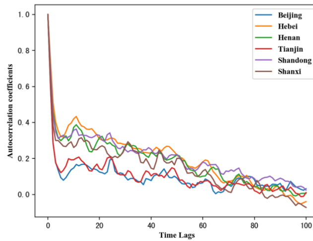
Fig. 4 The autocorrelation coefficients of different time lags
