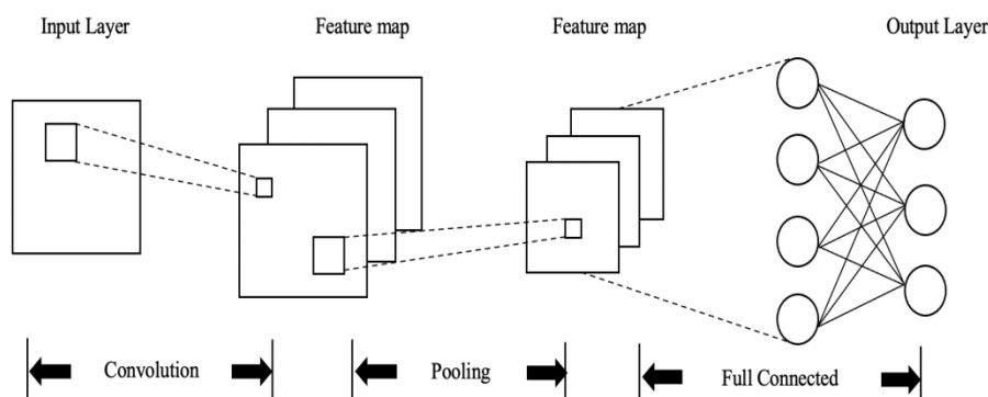
Fig. 6 The structure of simple convolutional neural network
