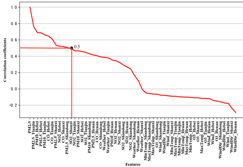
Fig. 3 The correlation coefficients of different features from surrounding cities
