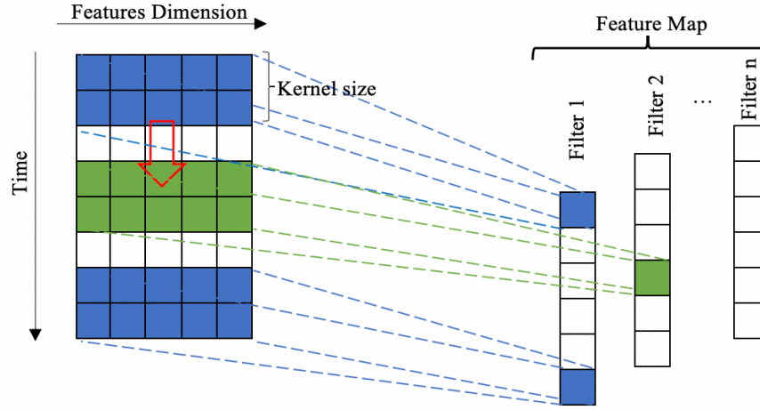
Fig. 7 The learning mechanism of 1D CNN
