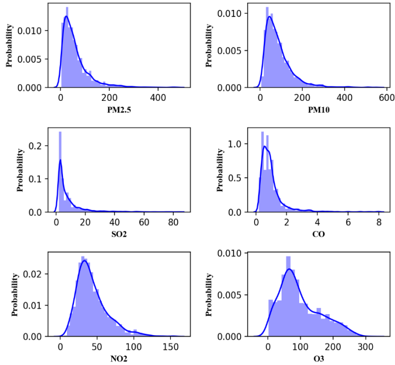
Fig. 2 The probability distribution of different continuous variables
