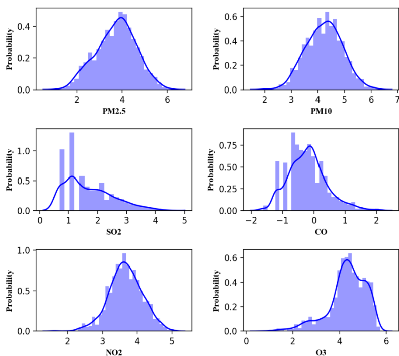
Fig. 11 The probability distribution of different continuous variables after logarithmic transformation
