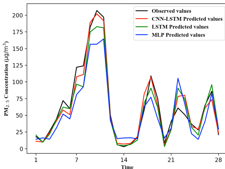
Fig. 12 Comparison of prediction results of different models
