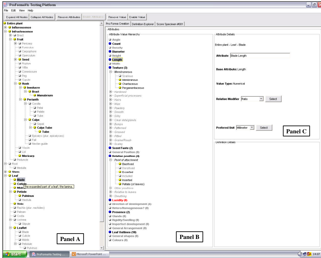
Figure 5: Specialisation Interface Screenshot. Panel A represents the Description Object Hierarchy. B represents the potential Attributes and their related possible values for a selected description object (The Attribute-Value Hierarchy). Panel C is an Attribute specification interaction object to allow finer control of the Attribute constraints and modifiers.
