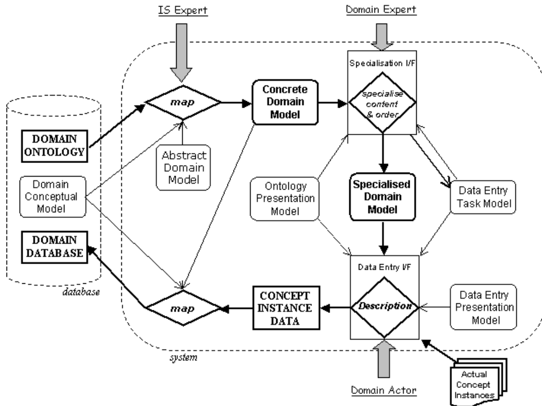
Figure 1: Ontology Driven Automated Generation Of Data Entry Interfaces To Databases Approach. In taxonomy, the domain expert and the domain actors are usually the same individual, though that is not a requirement of the approach.
