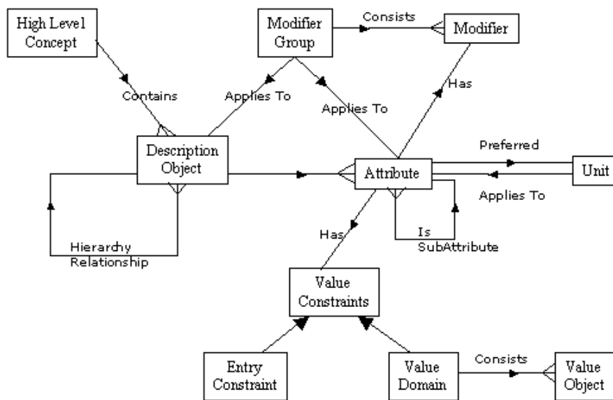
Figure 2: Abstract Domain Model. This is the conceptual model for controlling domain knowledge in the system. The hierarchy of Description Objects is formed using the Hierarchy Relationship. Some additional non-fundamental details, such as synonym relationships are not shown for clarity.
