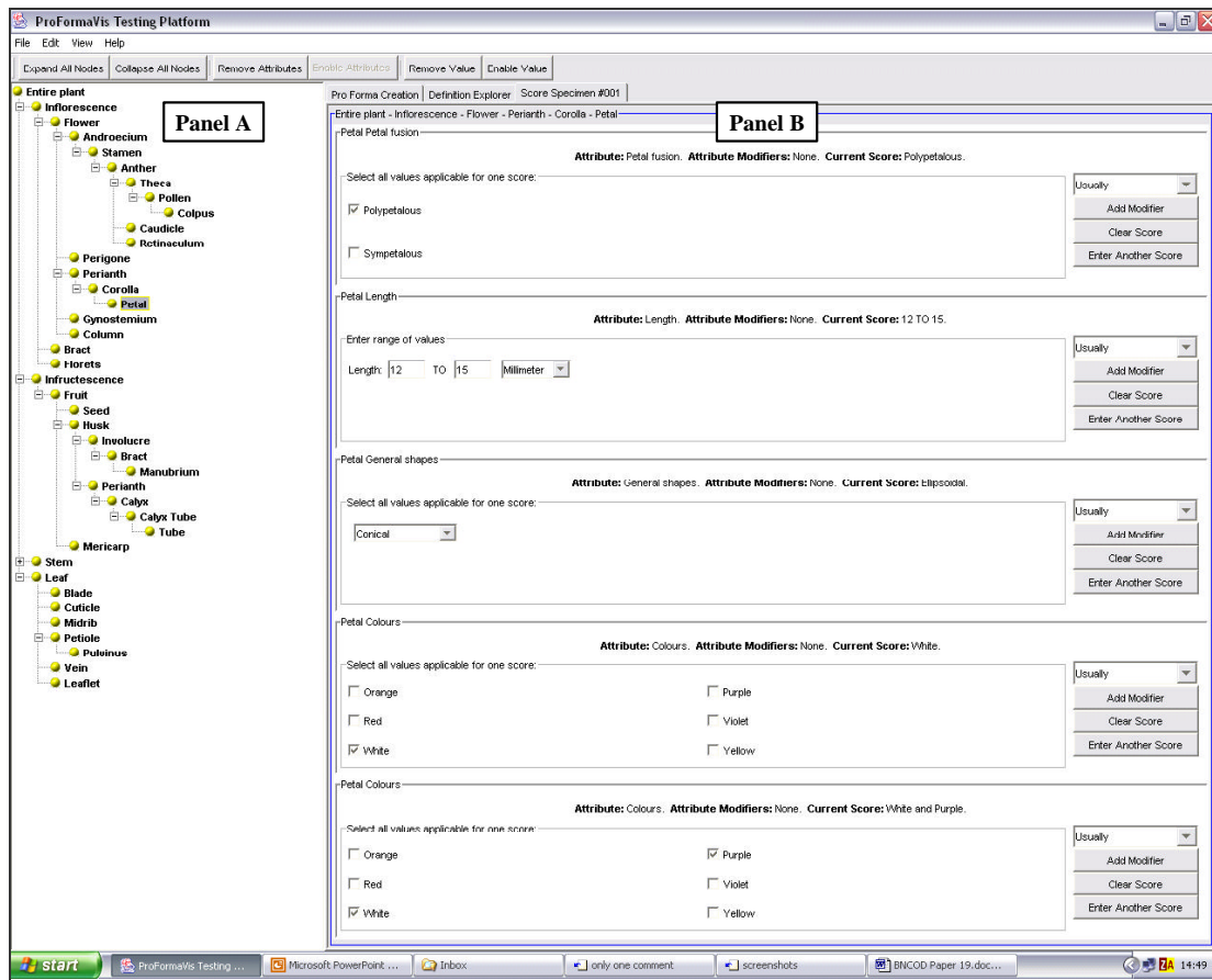
Figure 6: Data Entry Interface Example. 6A is the Description Object Hierarchy view (i.e. plant structures) providing both compositional context and a means of overriding the default data entry ordering. 6B is a group of Attribute Presentation Units for the selected Description Object (i.e. the structure with the compositional context Inflorescence-Perianth-Corolla-Petal). (The bottom two Attribute Presentation Units are copies of each other, as explained in the example in section 4.3 below,)
